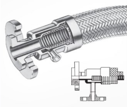
Heater and Coolant-Traced Hose
